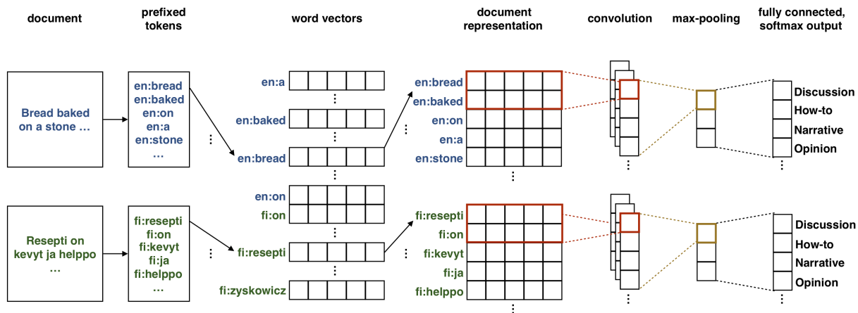
Figure 1: Illustration of text classification approach. Tokens are prefixed with language tags to differentiate e.g. the English word on from the Finnish word on ‘is’. Multilingual word vectors are used and the same network applied regardless of language to allow cross-lingual and multilingual training and classification. (Following in part Kim (2014))
