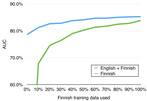
Figure 2: Average AUC for Finnish register prediction when training with varying proportions of Finnish training data, contrasting performance with and without additional English training data.
