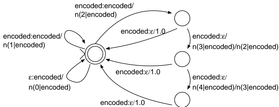
Figure 4: Fertility Model
