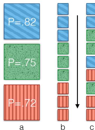
Figure 1: Sieve classifier decisions as ranked in a sieve architecture: (a) three sieves with their precisions, (b) each sieve’s decisions ranked as in a traditional system, (c) a potential ranking influenced by precision, but not strictly bound to it.
