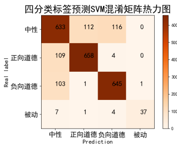
Figure 4: 四分类标签预测
